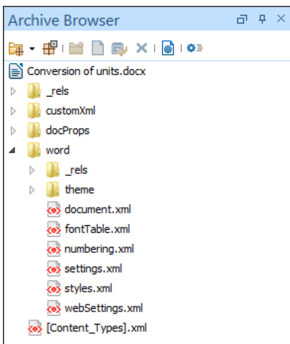
Figure 134. Archive Browser
