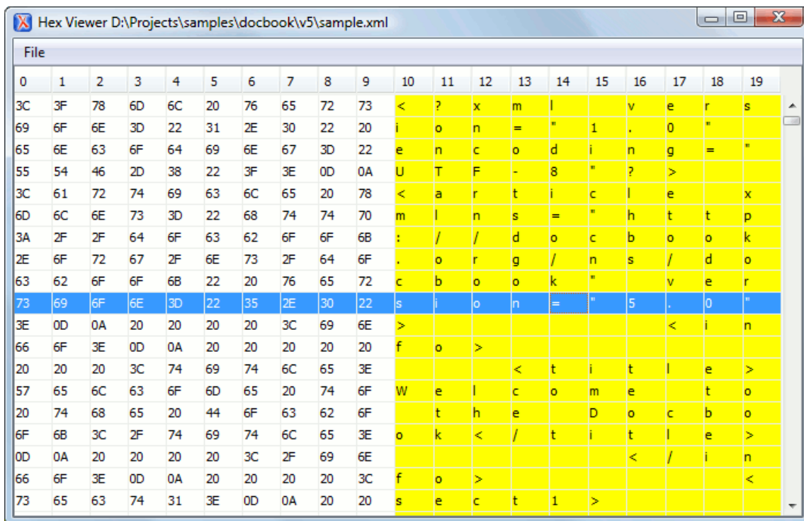
Figure 164. Hex Viewer
