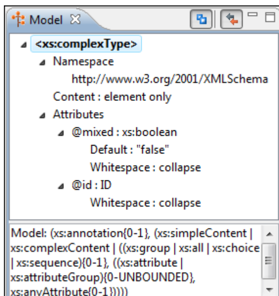
Figure 99. Element Structure Panel
