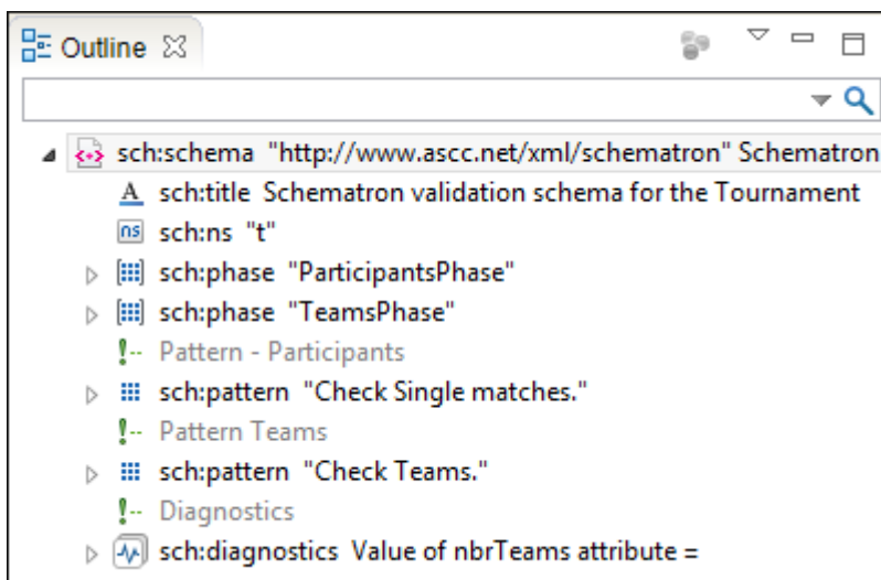
Figure 385. Schematron Outline View
