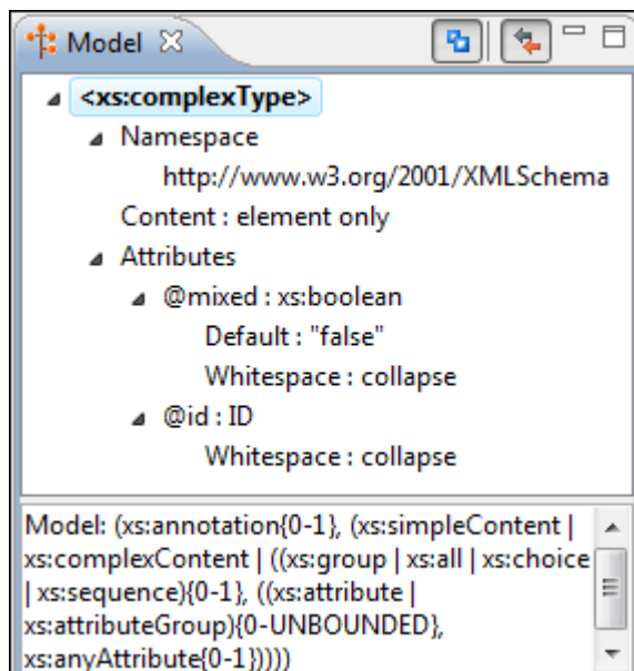
Figure 62. Element Structure Panel
