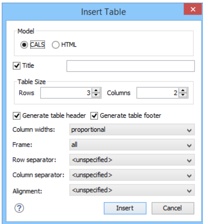
Figure 126. Insert Table Dialog Box - CALS Model
