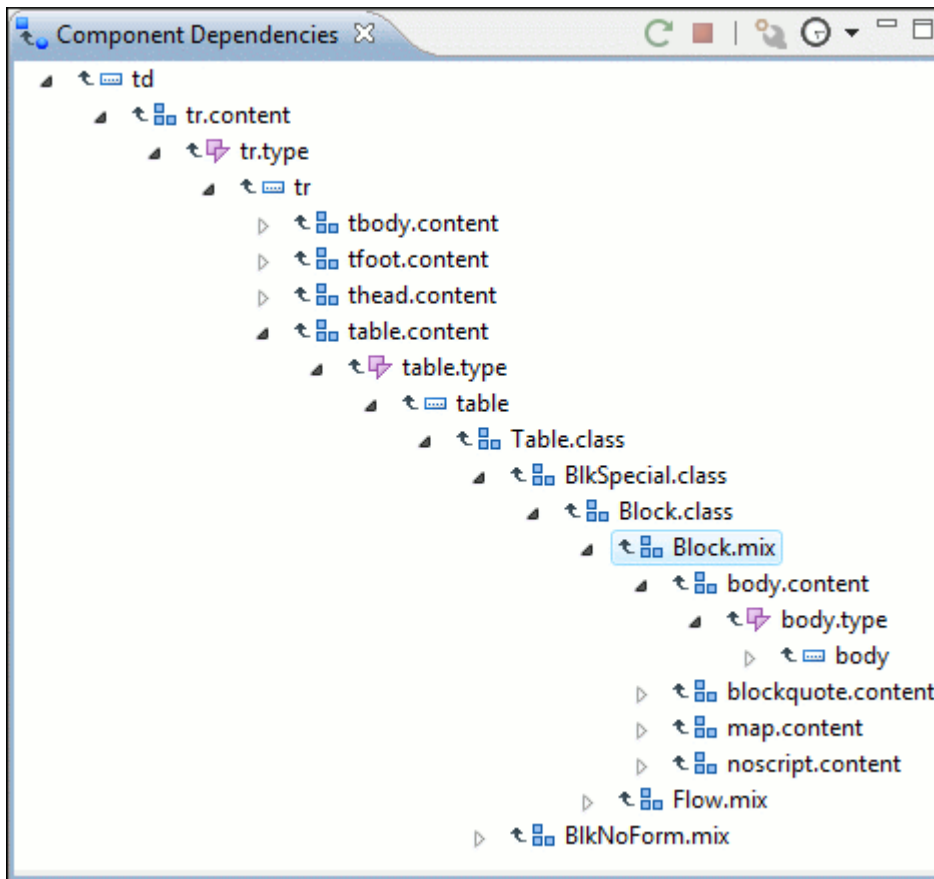
Figure 271. Component Dependencies View
