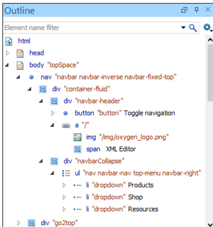
Figure 394. HTML Outline View
