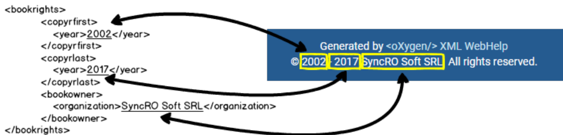
Figure 442. Example: Copyright Information Added in the WebHelp Footer
