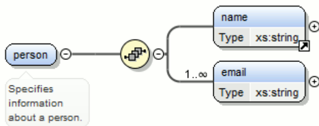
Figure 227. Extracting a Global Element
