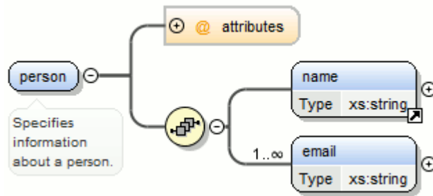
Figure 235. Extracting a Global Complex Type
