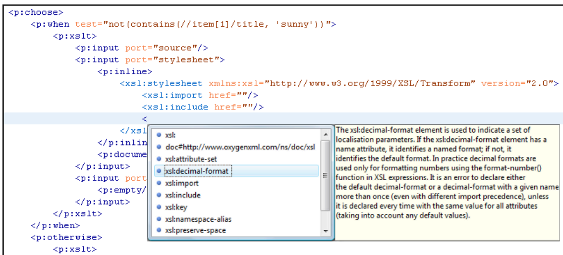
Figure 288. XProc Content Completion
