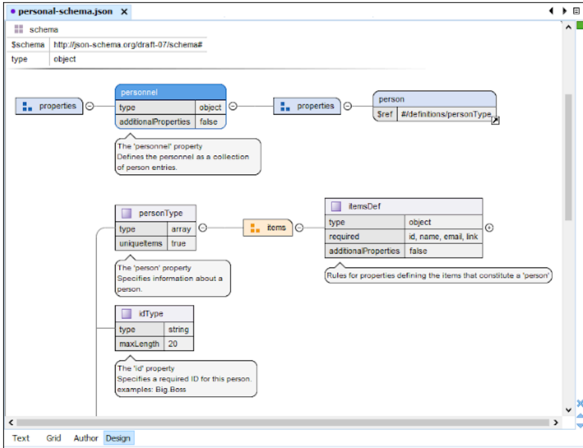
Figure 249. JSON Schema Design Mode
