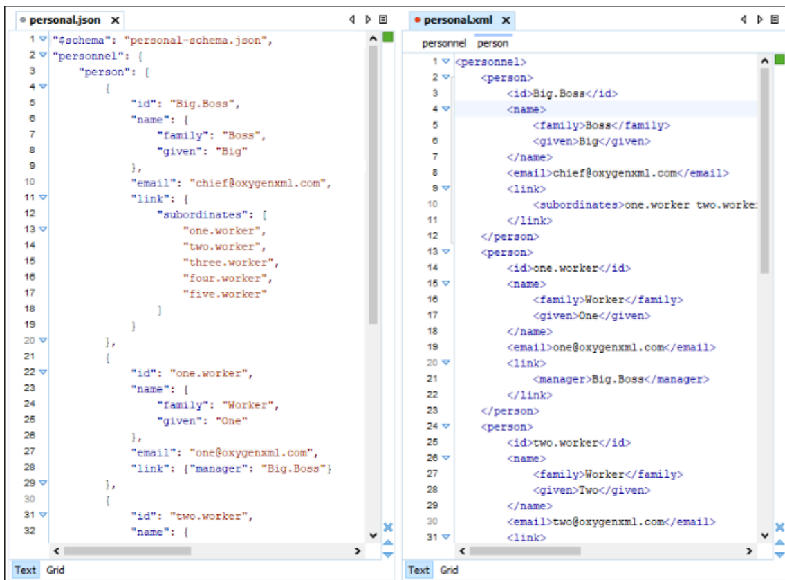
Figure 418. Example: XML to JSON Operation Result
