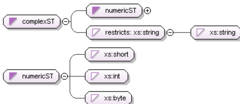
Figure 141. Extracting a Global Simple Type on a union Component
