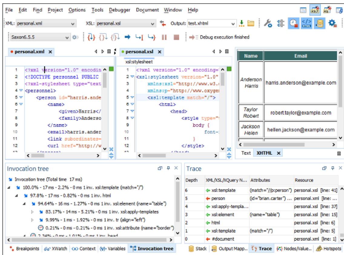
Figure 453. Debugger Interface
