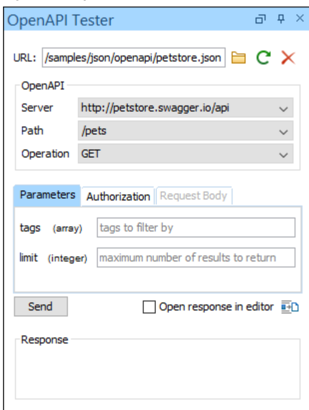
Figure 511. OpenAPI Tester View
