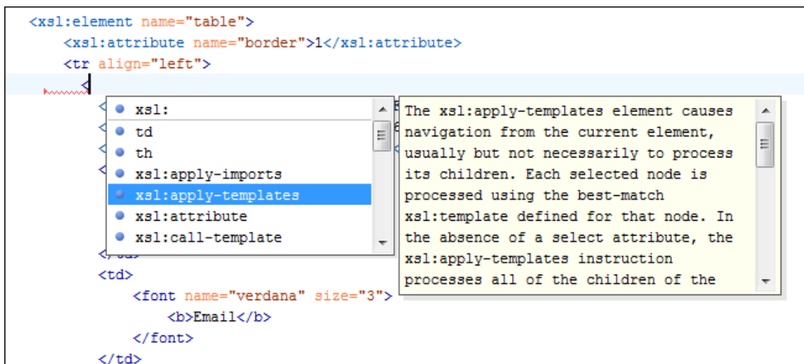
Figure 161. XSLT Content Completion Assistant
