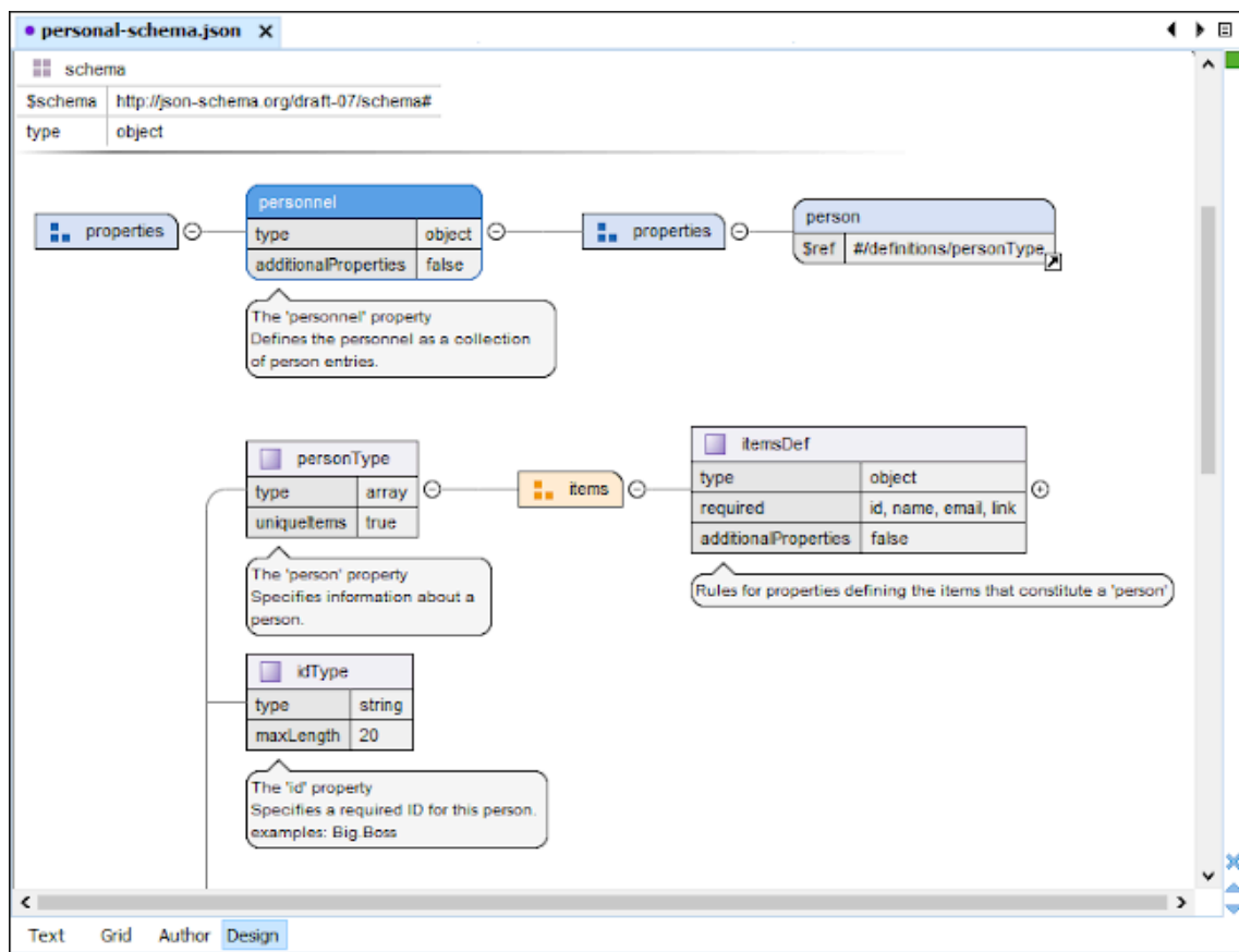
Figure 310. JSON Schema Design Mode
