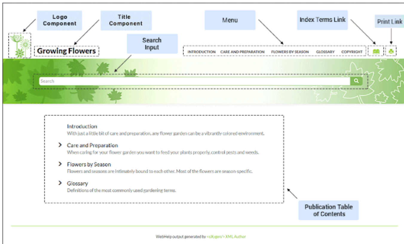
Figure 396. Examples of Main Page Components for a Tree Style of Layout
