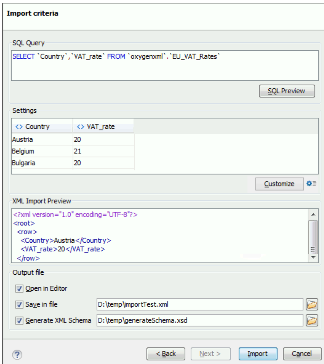
Figure 452. Import from Database Criteria Dialog Box
