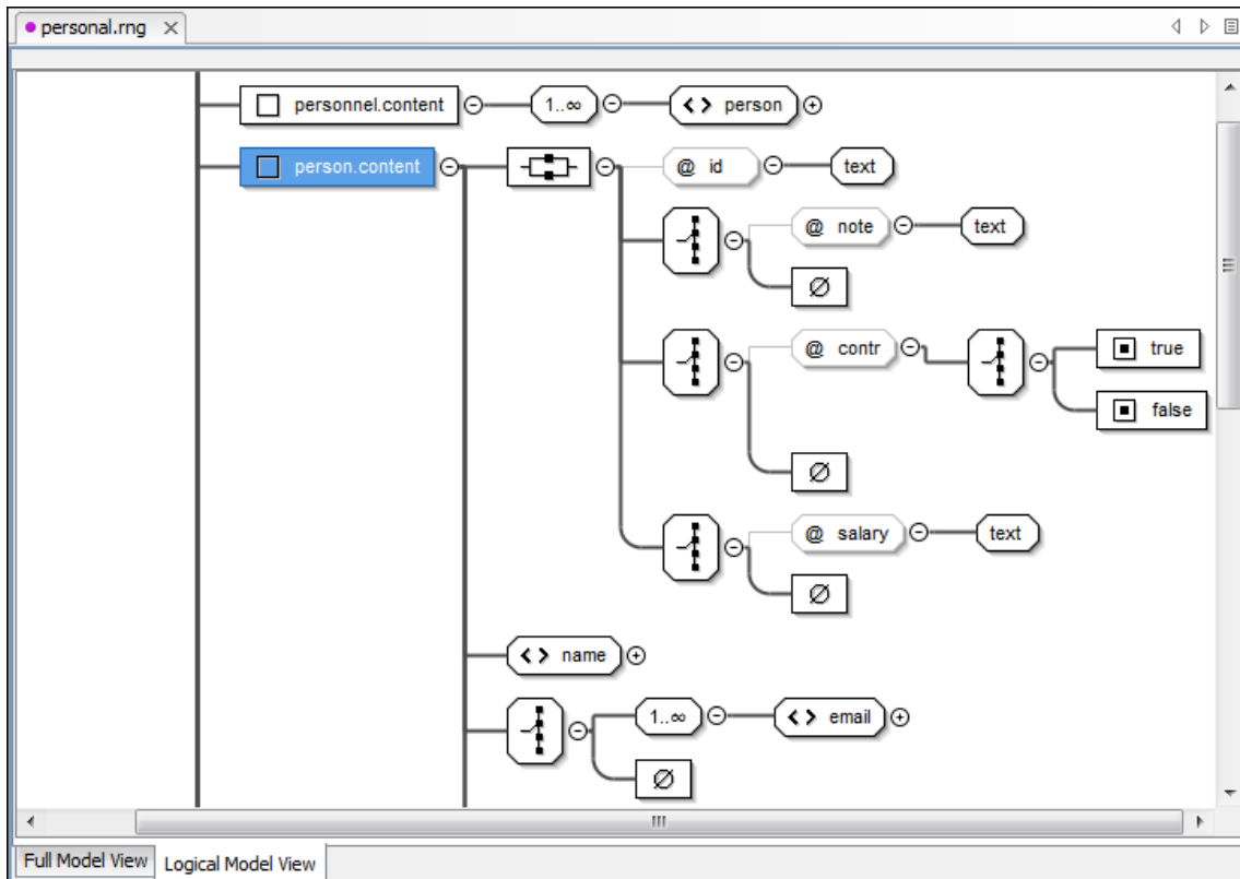
Figure 282. Logical Model View for a Relax NG Schema
