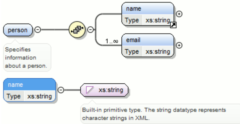
Figure 193. Extracting a Global Element on a <name> Element
