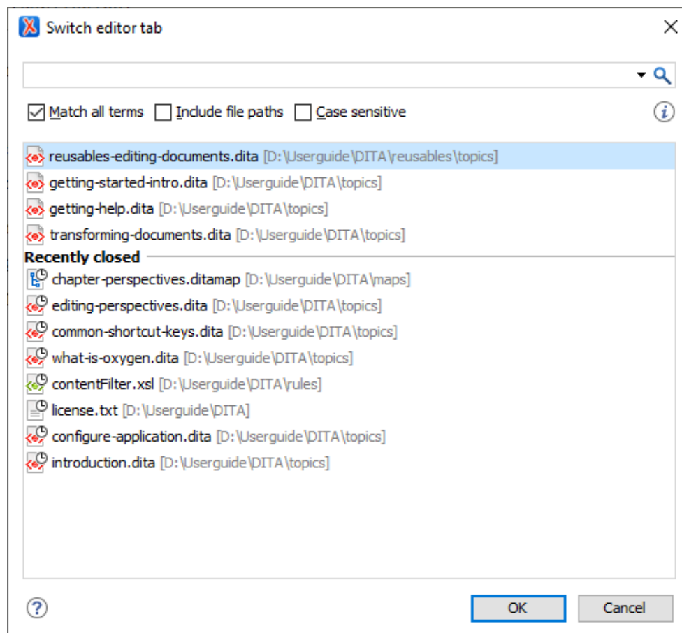
Figure 62. Switch Editor Tab Dialog Box
