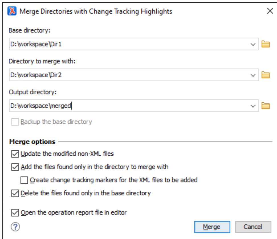
Figure 550. Merge Directories with Change Tracking Highlights Dialog Box
