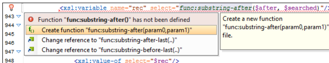
Figure 159. Example of an Undefined XSLT Functions Quick Fix
