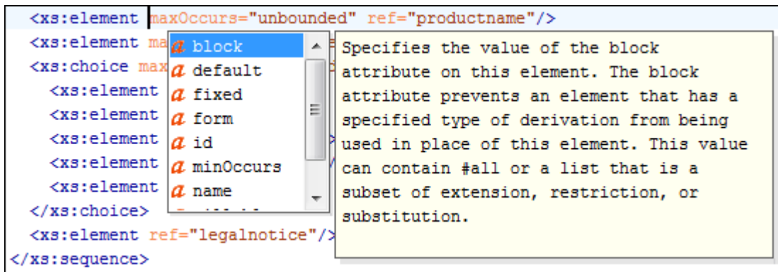
Figure 104. Content Completion Assistant
