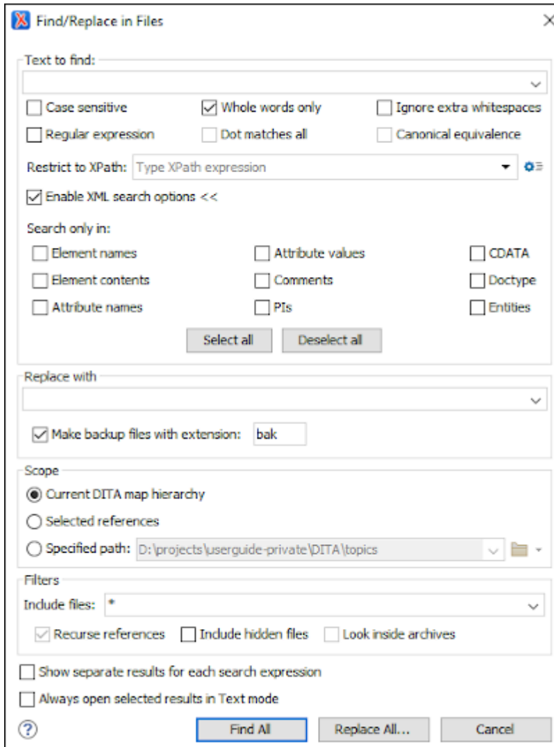
Figure 70. Find / Replace in Files Dialog Box (When Opened from the Toolbar Button)
