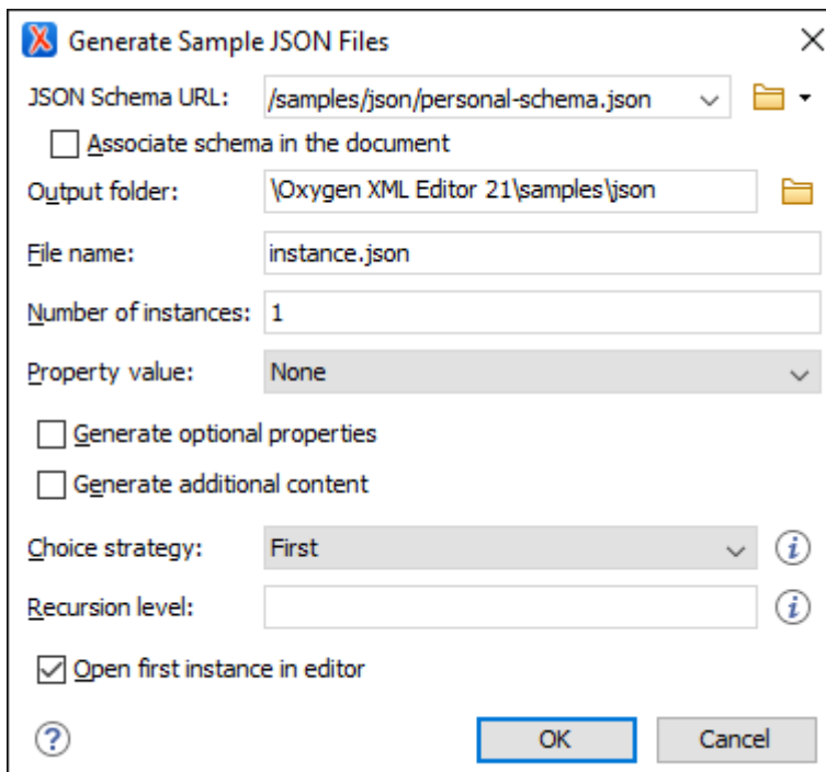
Figure 500. Generate Sample JSON Files Dialog Box
