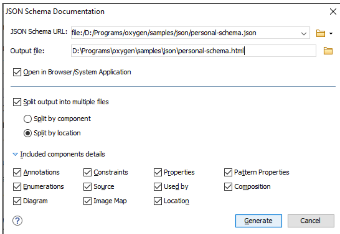
Figure 338. JSON Schema Documentation Dialog Box
