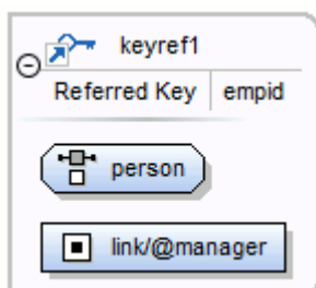
Figure 224. The xs:keyRef Component
