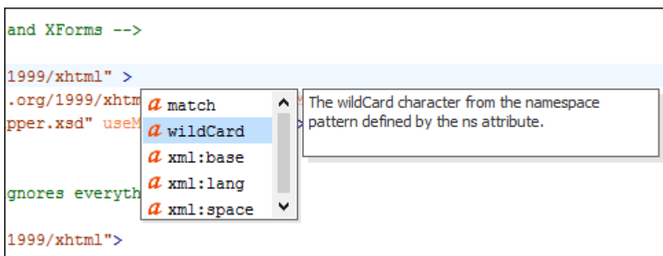
Figure 291. NVDL Content Completion Assistant
