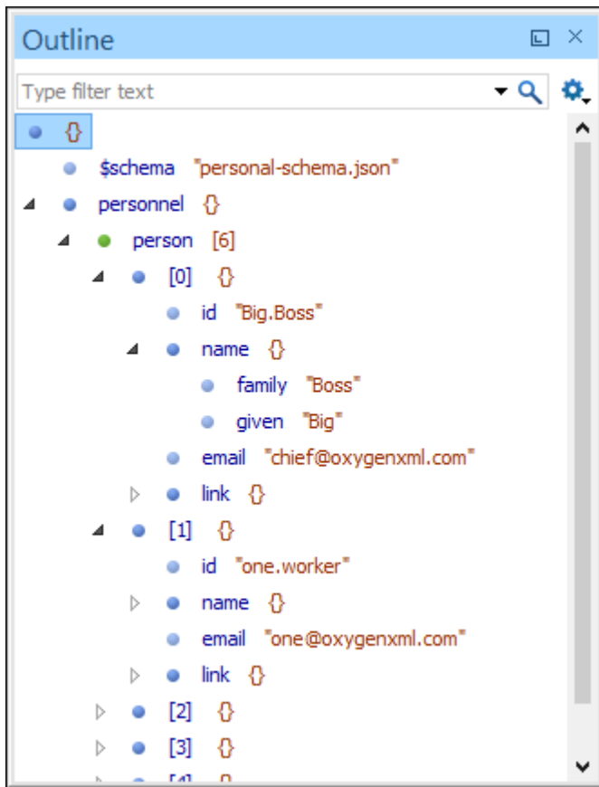
Figure 301. JSON Outline View
