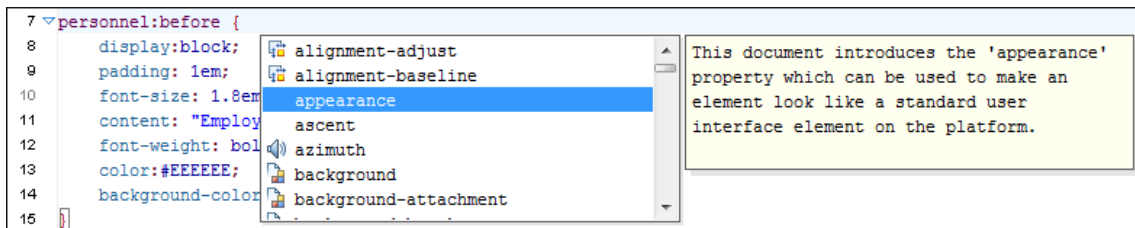
Figure 280. Content Completion in LESS Stylesheets
