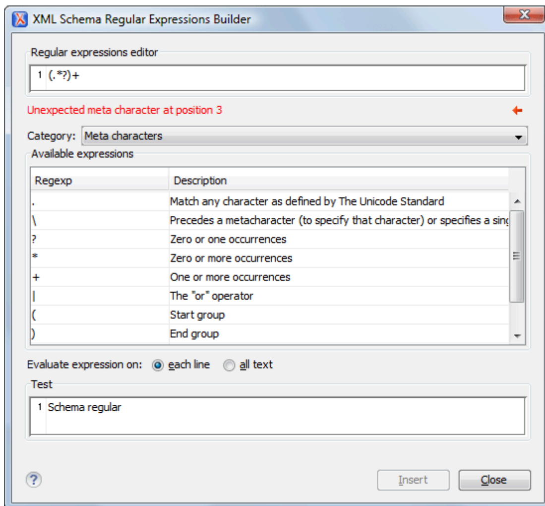
Figure 252. XML Schema Regular Expressions Builder Dialog Box
