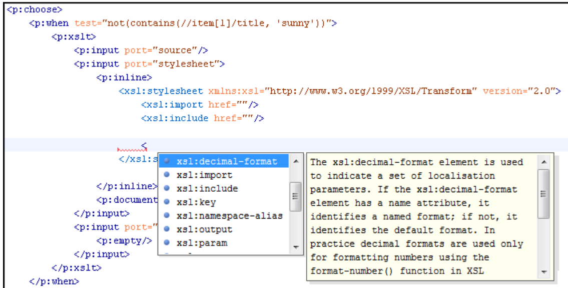
Figure 352. XProc Content Completion
