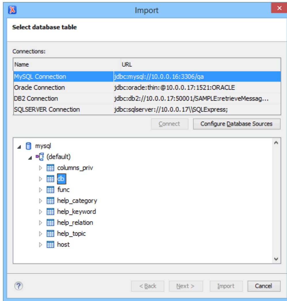
Figure 451. Select Database Table Dialog Box
