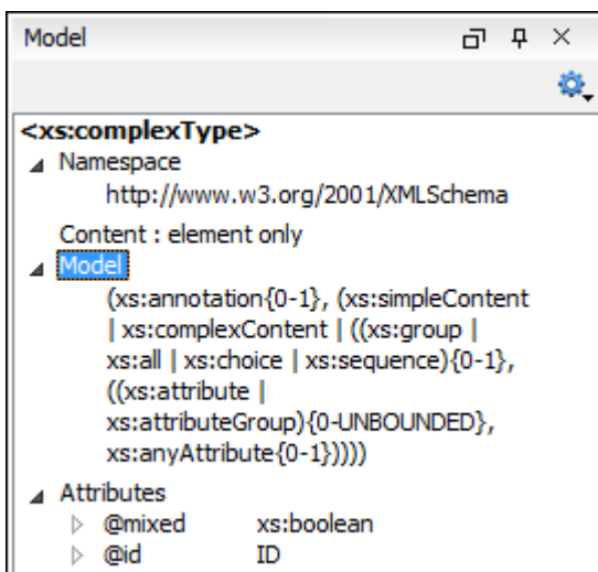
Figure 109. Element Structure Panel
