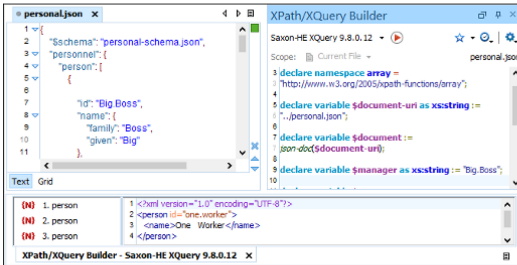
Figure 309. XPath/XQuery Builder View for JSON
