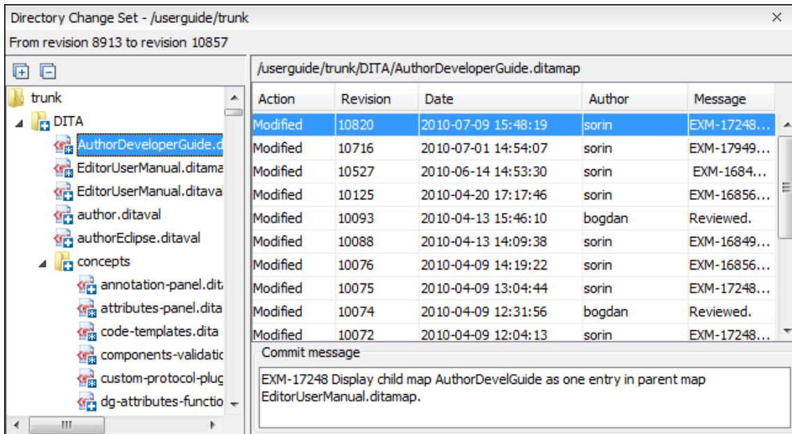
Figure 594. Directory Change Set View
