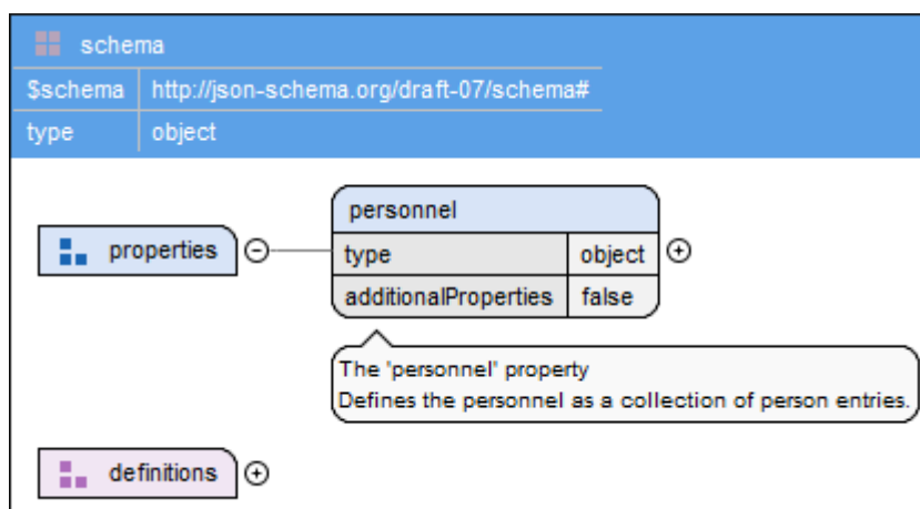
Figure 315. The schema Component
