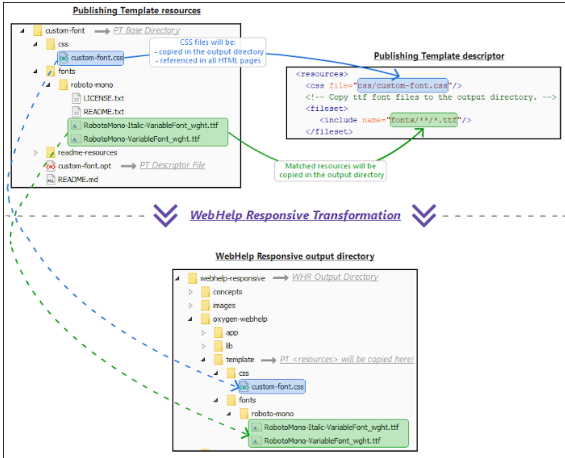
Figure 408. Referencing Local Fonts in a Publishing Template
