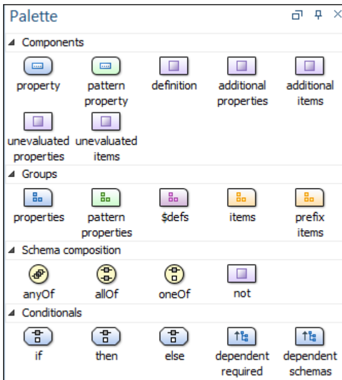
Figure 312. JSON Palette View (for schema versions 2019-09, 2020-12)
