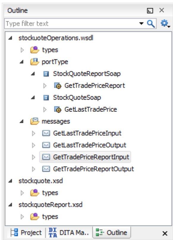
Figure 266. WSDL Outline View
