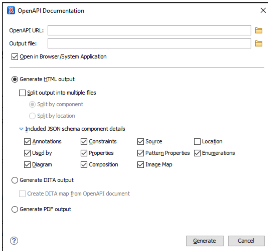
Figure 523. OpenAPI Documentation Dialog Box
