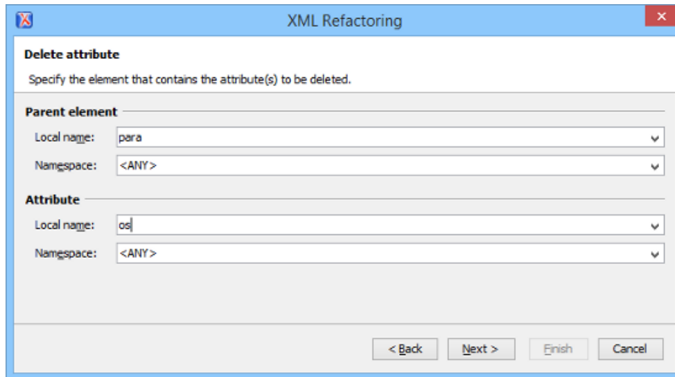
Figure 149. XML Refactoring 2nd Wizard Page (Delete Attribute Operation)
