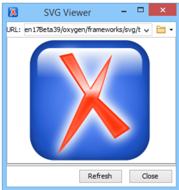
Figure 362. SVG Viewer
