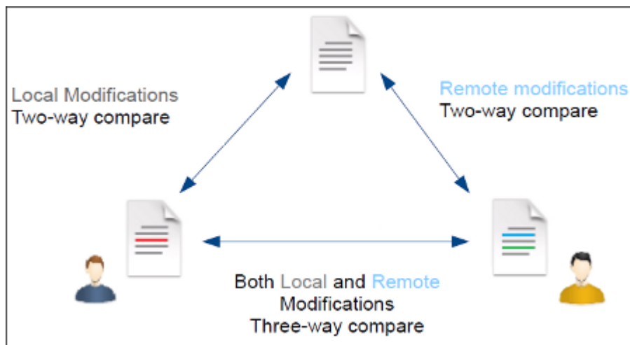
Figure 534. Three-Way Comparison
