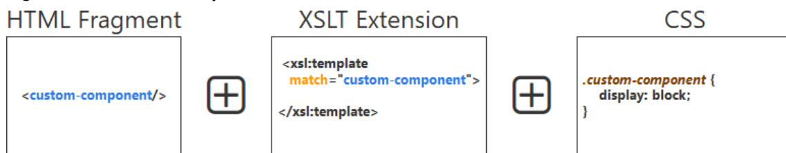
Figure 406. Custom Component
