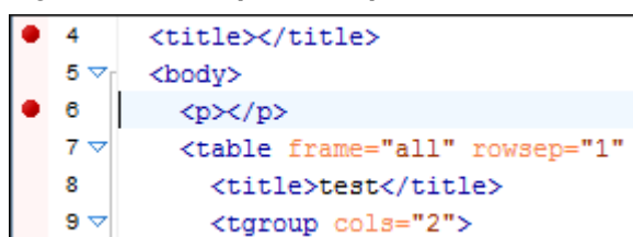
Figure 469. Example: Breakpoints
