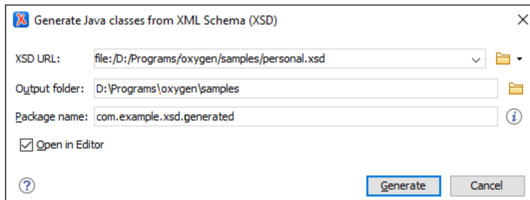
Figure 498. Generate Java Classes from XML Schema (XSD) Dialog Box
