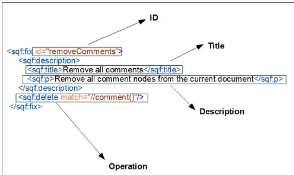
Figure 360. Schematron Quick Fix Components
