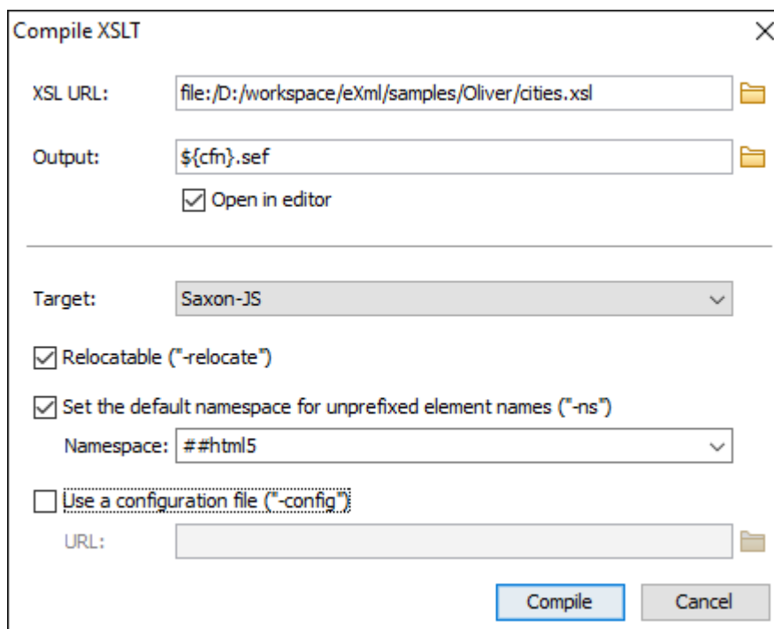
Figure 499. Compile XSLT Stylesheet for Saxon Dialog Box
