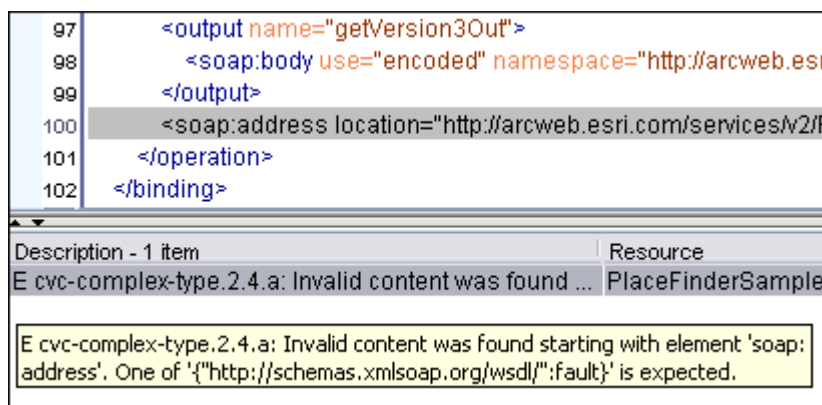
Figure 263. Validating a WSDL file
