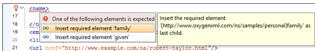
Figure 138. Quick Fix Menu Invoked by Clicking on the 💡 Icon
