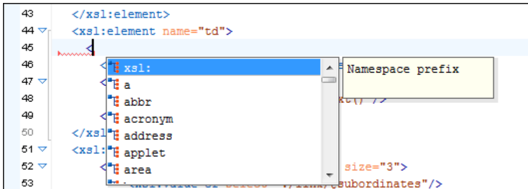
Figure 162. Namespace Prefixes in the Content Completion Assistant
