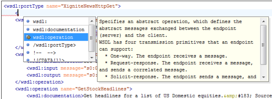
Figure 264. WSDL Content Completion Assistant
