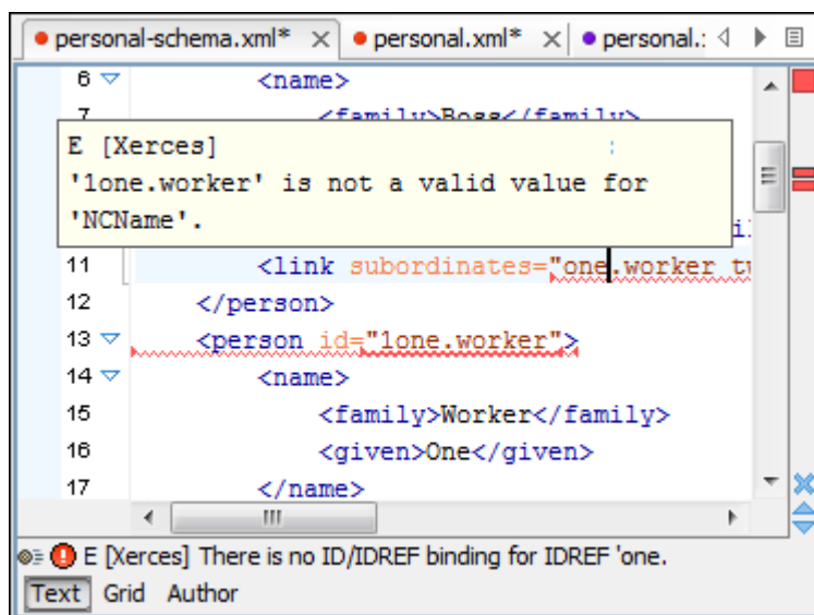
Figure 125. Presenting Validation Errors in Text Mode
