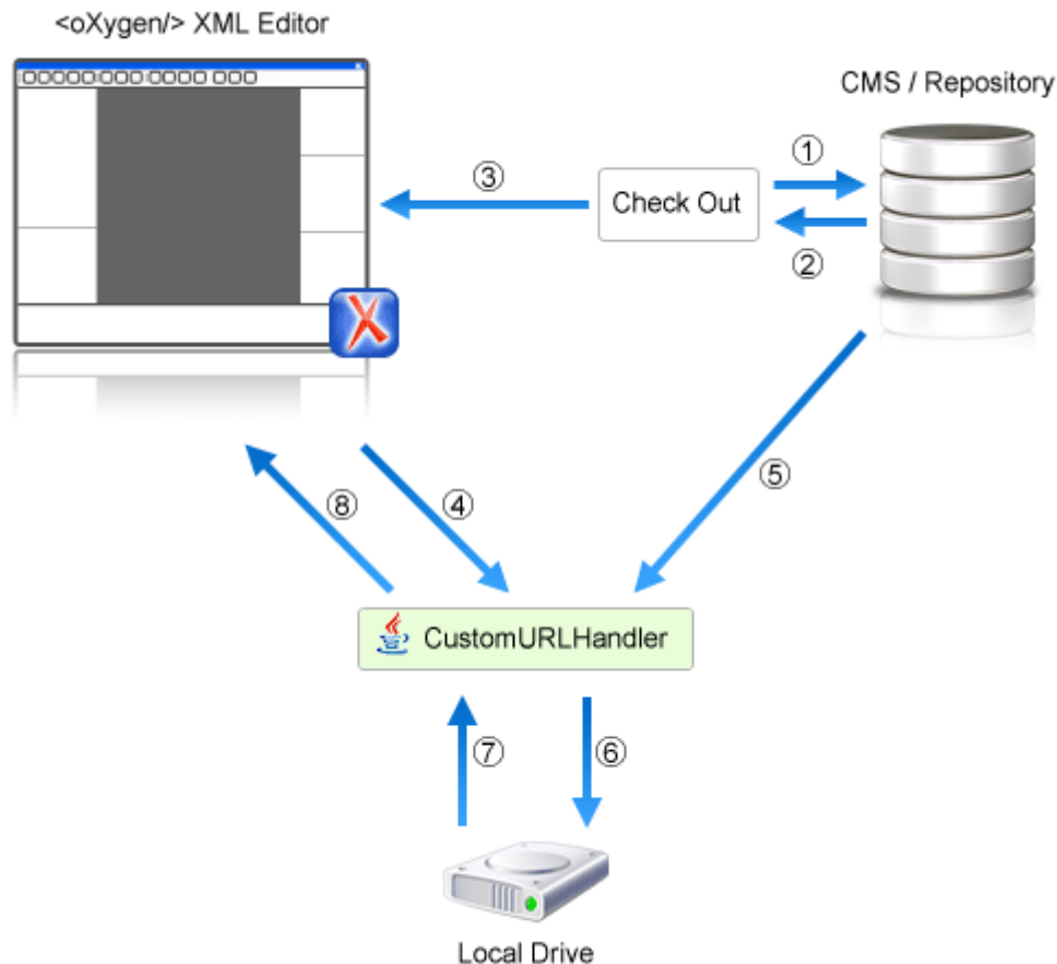
Figure 473. Check Out Process Diagram
