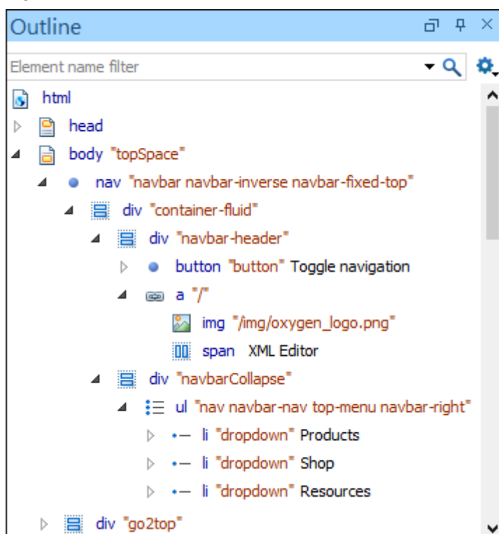
Figure 365. HTML Outline View
