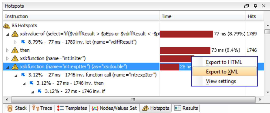
Figure 472. Hotspots View
