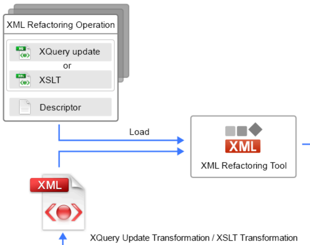
Figure 151. Diagram of an XML Refactoring Operation
