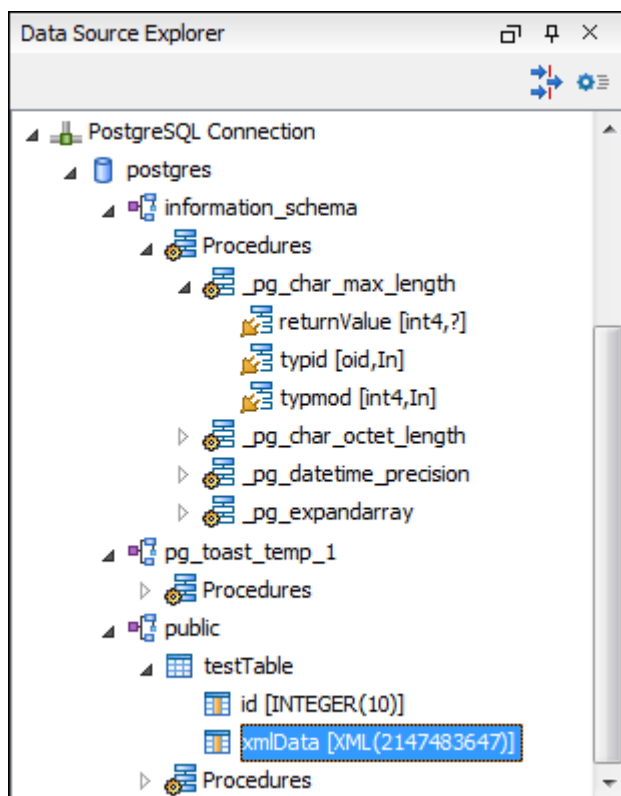
Figure 432. PostgreSQL Database Connection
