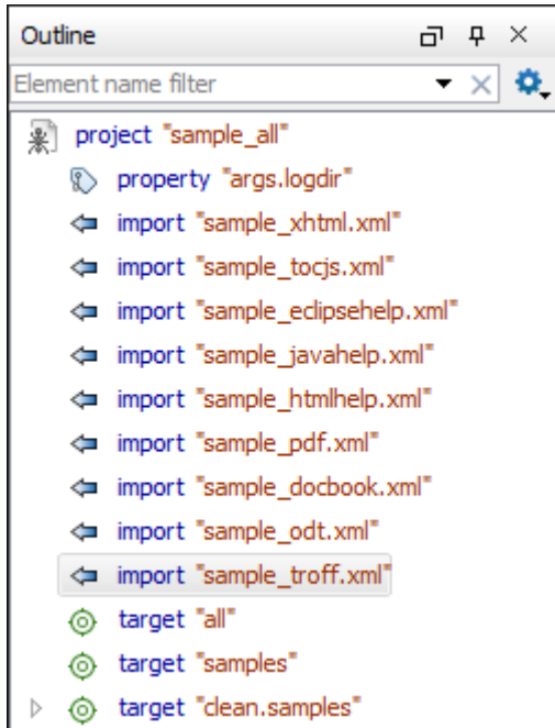
Figure 187. Ant Outline View
