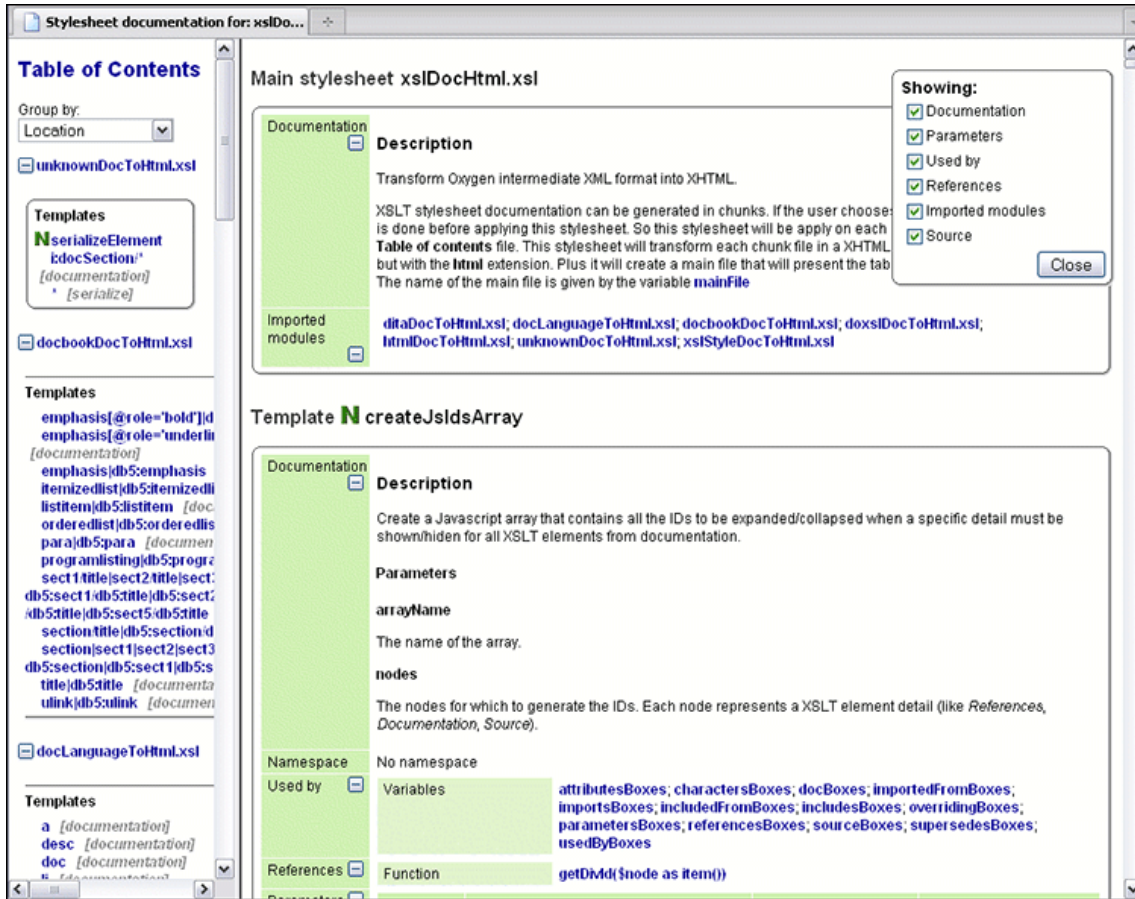
Figure 181. XSLT Stylesheet Documentation Example
