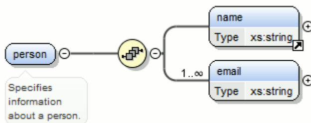
Figure 196. Extracting a Global Group
