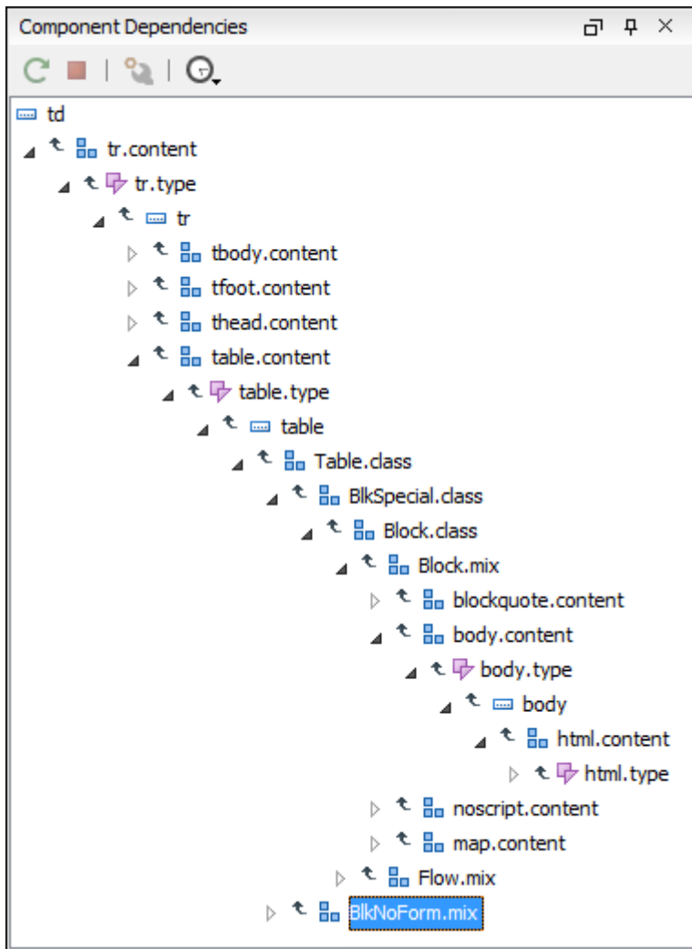
Figure 236. Component Dependencies View
