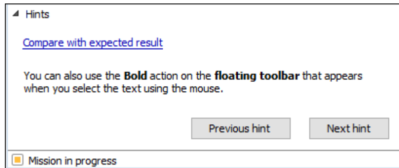
Figure 478. Hints Pane
