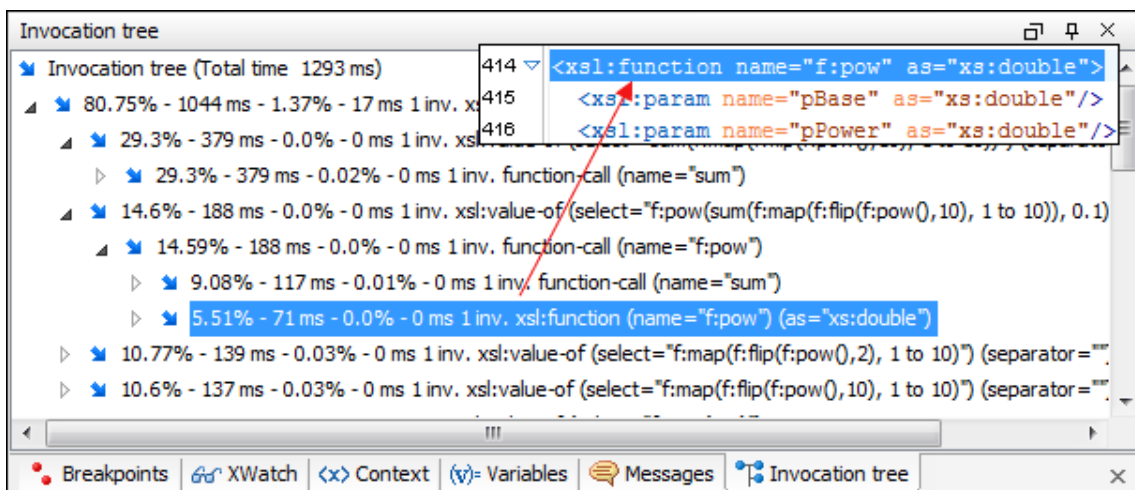
Figure 470. Source Backmapping
