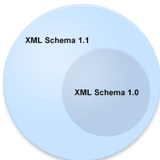
Figure 253. XML Schema 1.1
