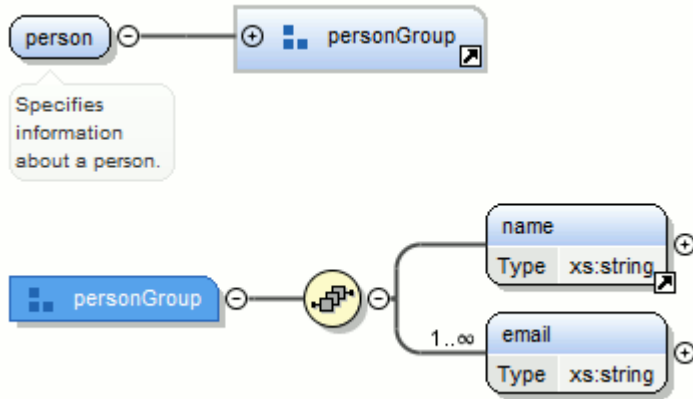
Figure 197. Extracting a Global Group on a <sequence> Element
