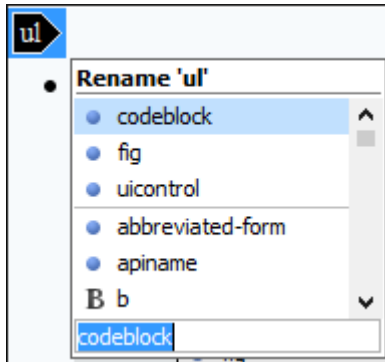
Figure 89. Example (Rename)
