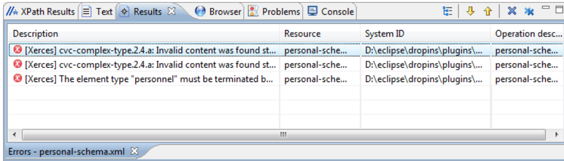
Figure 65. Results View
