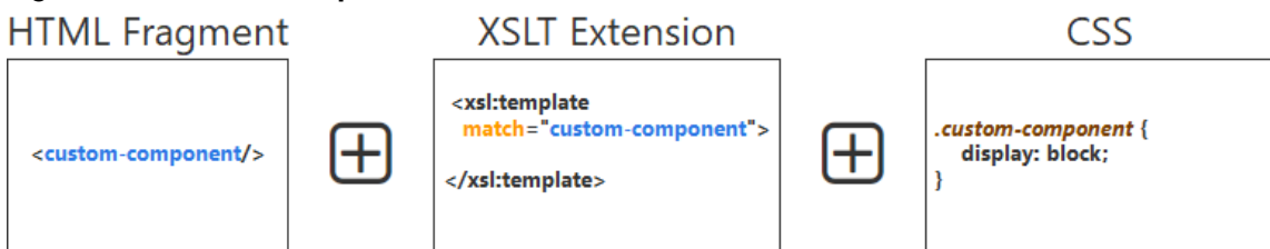
Figure 242. Custom Component
